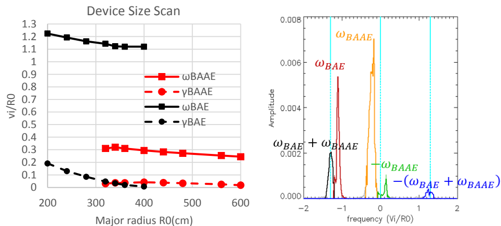
Fig. a) Frequencies (solid) and growth rate (dash) of BAAE (red) and BAE (black) when the major radius R_0 changes. b) Fourier transform of the electron potential, the spectrum are discrete with BAAE (orange), BAE (red), beating wave (black), negative BAAE (green) and beating wave (blue), R_0=340 cm
